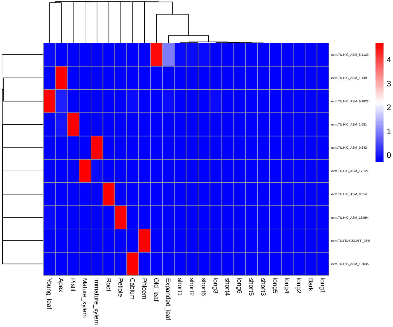
Expression of Hub Genes (Z-score normalized)
